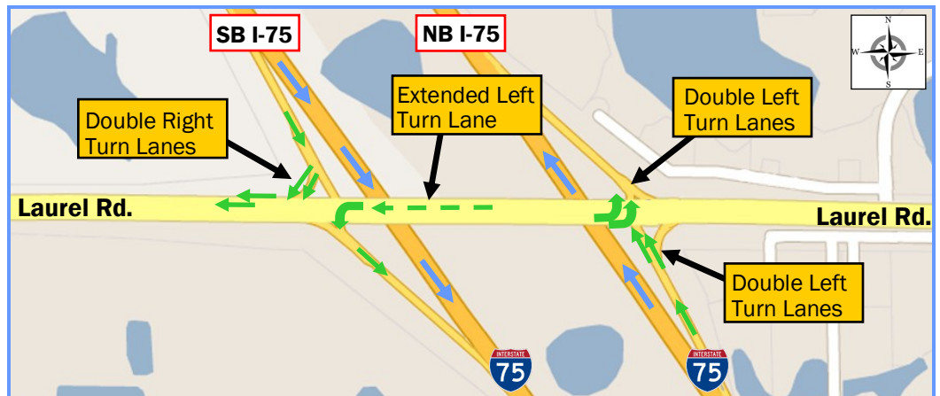
FIGURE 1: LAUREL ROAD AND I-75 INTERCHANGE IMPROVEMENTS
